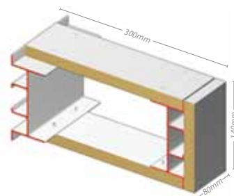
XPP1-030 Pelmet Pod
