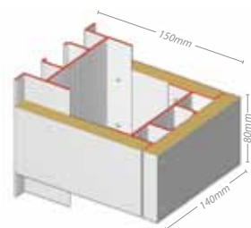
XMP1-015 Mullion Pod (Suitable for a 50mm cavity wall)
