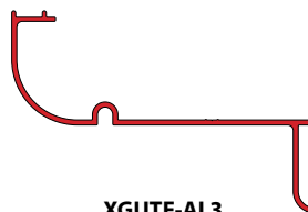
XGUTF-AL3 Aluminium Gutter Fascia Bottom Section
